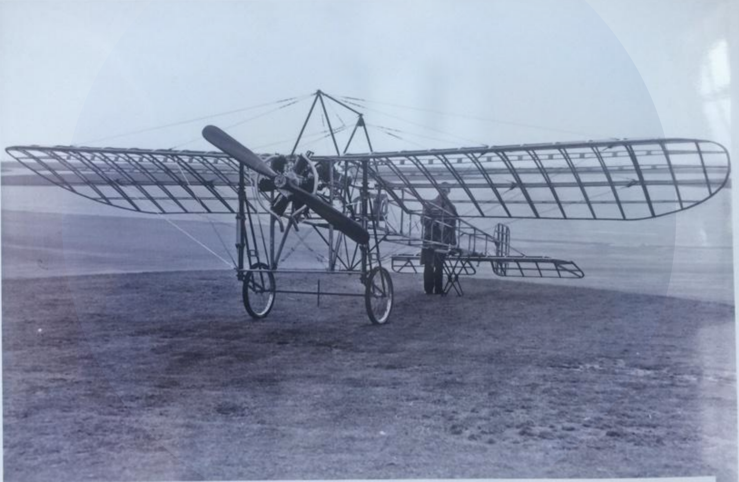
BLERIOT AIRCRAFT RECONSTRUCTED BY ENGINEERING WING WORKSHOP
